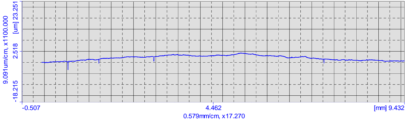
Profil=P_ISO - Section=[1]
