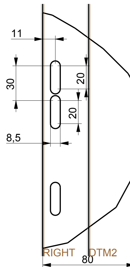
DETAIL A SCALE 0,500
