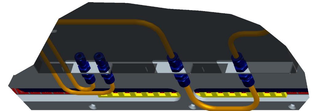
DETAIL C SCALE 0,300
