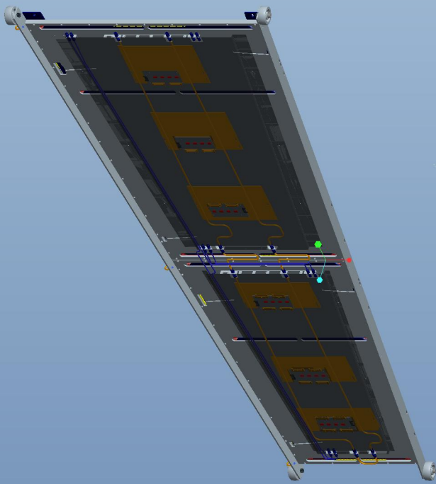
Active Piping Asm:RE4-R2-R3-FRAME
