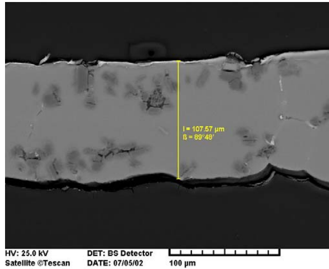
Fig. 11. Clustering of spinel coated \text{Al}_2\text{O}_3 particles in aluminium foam with low Si/Mg ratio, cell wall cross-section, SEM picture.
