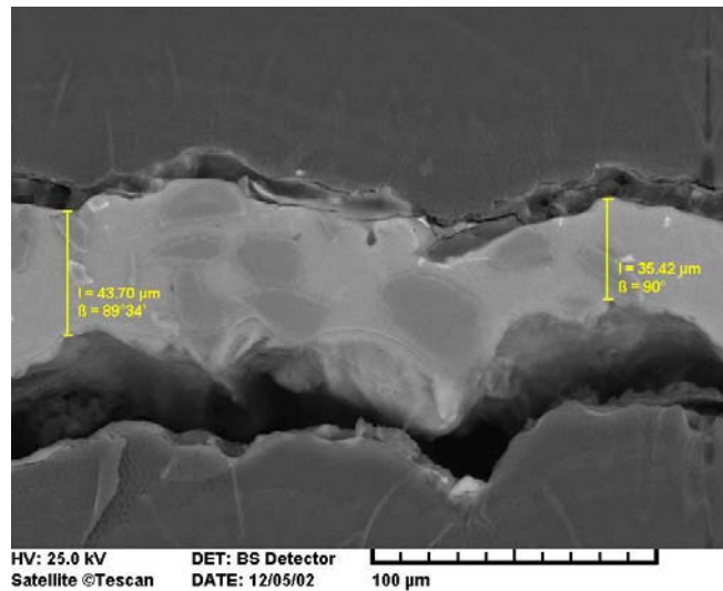
Fig. 12. Single spinel free \text{Al}_2\text{O}_3 particles in aluminium foam with high Si/Mg ratio, cell wall cross-section, SEM picture.
