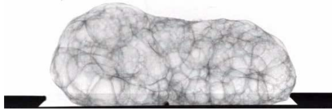
Fig. 2. Liquid-Al foam stabilised with 13 \mu\text{m} SiC particles produced from “Formgrip” precursors containing \text{AlSi9Cu3} + 10 \text{ vol.\% SiC} and 0.5 wt% \text{TiH}_2 as blowing agent, real-time X-ray radiography picture was obtained using a synchrotron beam.
