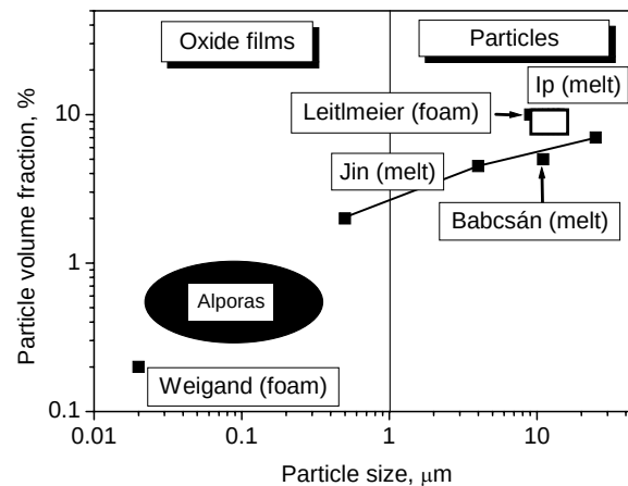
Fig. 9. Speculative stability diagramme for metal foams relating particle volume fraction and particle size. Data given by various authors measured in the foam or in the melt are included.
