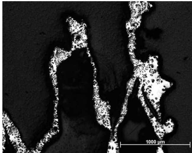
Fig. 10. Irregular metallic bubble remnants produced when foaming aluminium alloy reinforced with \text{TiB}_2 particles. A cross section of the remnants is shown with optical microscopy.
