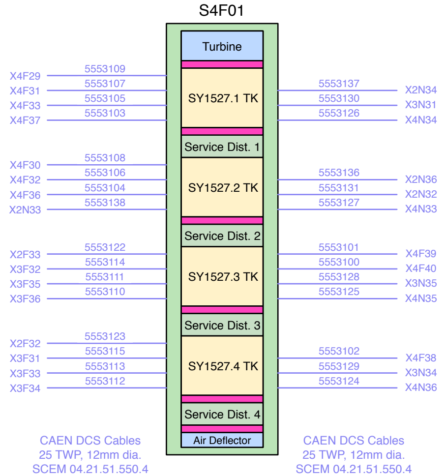
DCS Cabling
