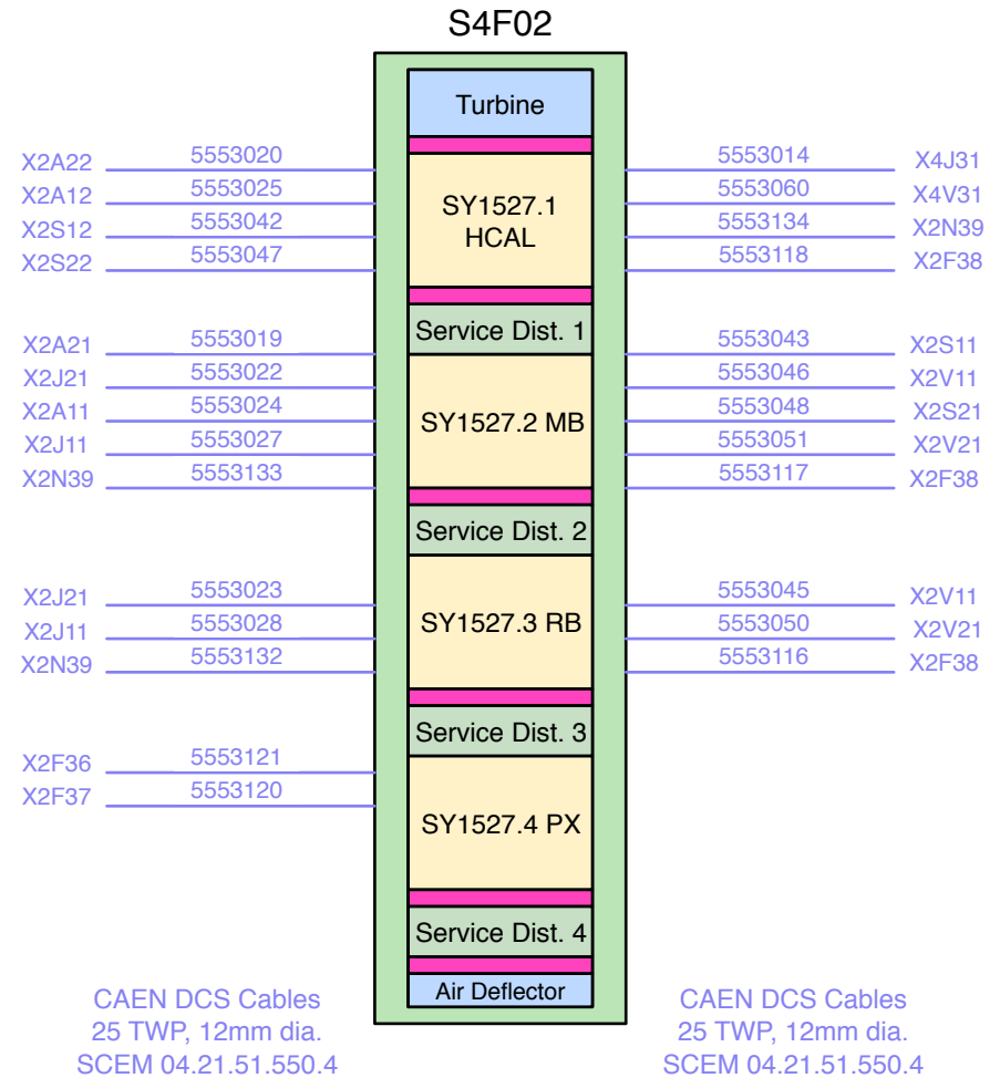
DCS Cabling
