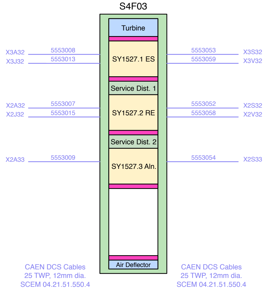
DCS Cabling
