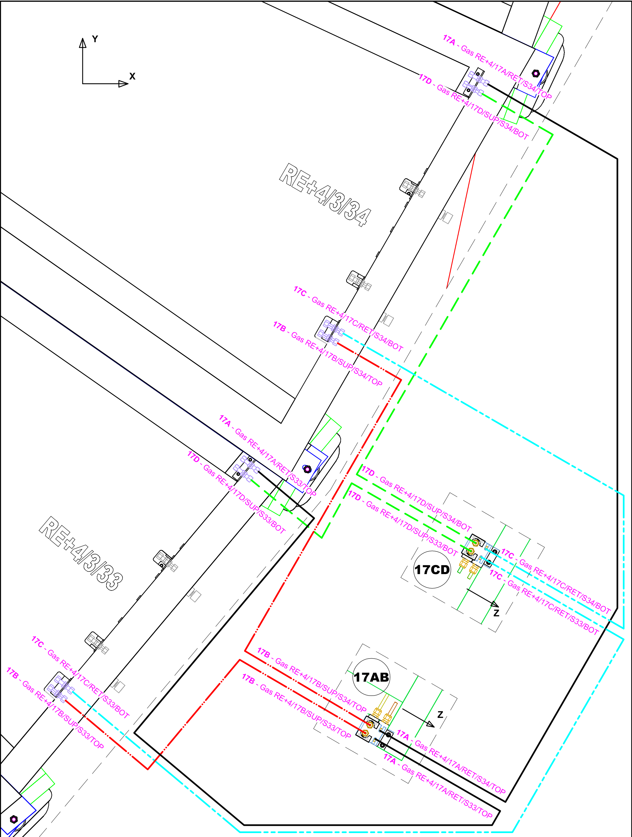
YE+3 ENDCAP Scheme of RPC RE+4 gas pipes connections from patchpanels to chambers Patchpanels 17AB, 17CD v.01 6.11.2013
